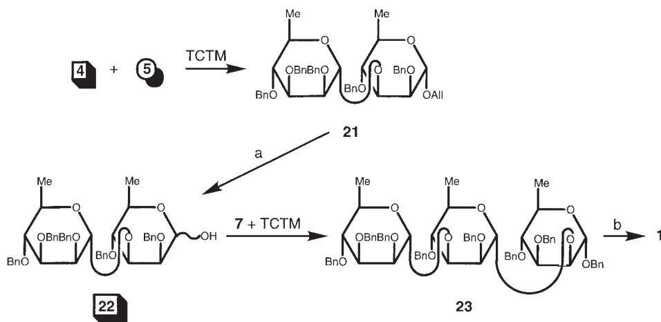
Fig. 4. Synthesis of \alpha\text{-D-Rhap-(1} \rightarrow 3\text{)-}\alpha\text{-D-Rhap-(1} \rightarrow 2\text{)-D-Rhap-OH (1)} (TCTM = \text{Me}_3\text{SiBr} + \text{CoBr}_2 + n\text{-Bu}_4\text{NBr} + \text{MS4A} ): a. \text{PdCl}_2 + \text{NaOAc}/\text{aq AcOH} (95%), rt; b. \text{H}_2 , Pd-C(10%)/MeOH, rt.
