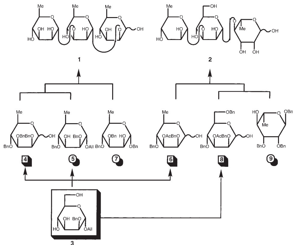
Fig. 1. Synthetic scheme for \alpha -D-Rhap-(1 \rightarrow 3)- \alpha -D-Rhap-(1 \rightarrow 2)-D-Rhap-OH ( 1 ) and \alpha -D-Tyvp-(1 \rightarrow 3)- \alpha -D-Manp-(1 \rightarrow 4)-L-Rhap-OH ( 2 ). A code with square shade is a donor, whereas that with round shade is an acceptor.
