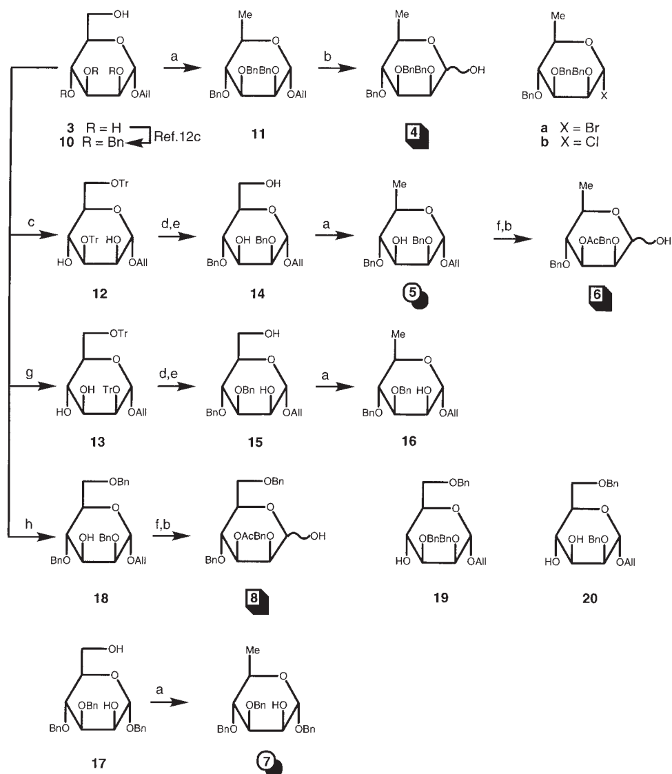
Fig. 3. Synthesis of partially benzylated D-rhamnose derivatives: a. (i) TsCl + pyridine (Py), -10^{\circ}\text{C} \rightarrow \text{room temperature (rt)} , (ii) \text{LiAlH}_4/\text{Et}_2\text{O} , 0^{\circ}\text{C} \rightarrow \text{reflux} ; b. \text{PdCl}_2 + \text{NaOAc}/\text{aq AcOH} (95%), rt; c. TrCl (2.3 eq) + Py, 55^{\circ}\text{C} ; d. BnBr + NaH/DMF, 0^{\circ}\text{C} \rightarrow \text{rt} ; e. \text{CF}_3\text{CO}_2\text{H} + \text{MeOH}/\text{CHCl}_3 , rt; f. \text{Ac}_2\text{O} + \text{Py} , rt; g. TrCl (3.0 eq) + Py, 100^{\circ}\text{C} ; h. BnCl + KOH, 140^{\circ}\text{C} .
