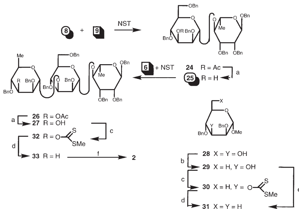
Fig. 5. Synthesis of \alpha -D-Tyvp-(1 \rightarrow 3)- \alpha -D-Manp-(1 \rightarrow 4)-L-Rhap-OH ( 2 ) (NST = NsCl + AgOTf + Et 3 N): a. dil NaOMe, rt; b. (i) TsCl + Py, -10^\circ\text{C} \rightarrow \text{rt} , (ii) LiAlH 4 /Et 2 O, 0^\circ\text{C} \rightarrow \text{reflux} ; c. (i) NaH/THF, rt, (ii) CS 2 /THF, rt, (iii) MeI/THF, rt; d. n -Bu 3 SnH + AIBN(cat.)/PhMe, N 2 , 110^\circ\text{C} ; e. (i) Tf 2 O + Py/CH 2 Cl 2 , -30^\circ\text{C} \rightarrow 20^\circ\text{C} , (ii) n -Bu 4 NBH 4 /PhMe, 50^\circ\text{C} ; f. H 2 , Pd-C(10%)/MeOH, rt.
