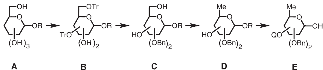
Fig. 2. A route to partially benzylated 6-deoxyhexoses.
